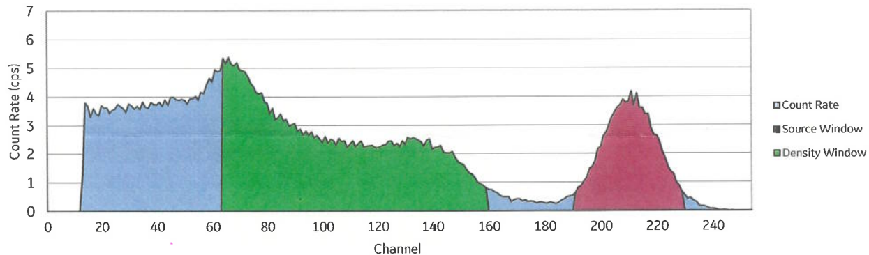
Elevated Temperature Spectrum
