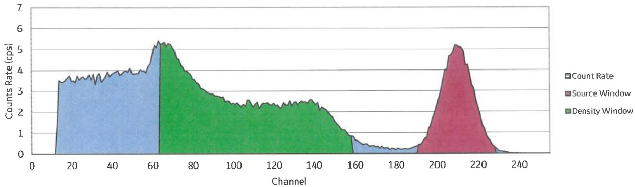
Ambient Temperature Spectrum
